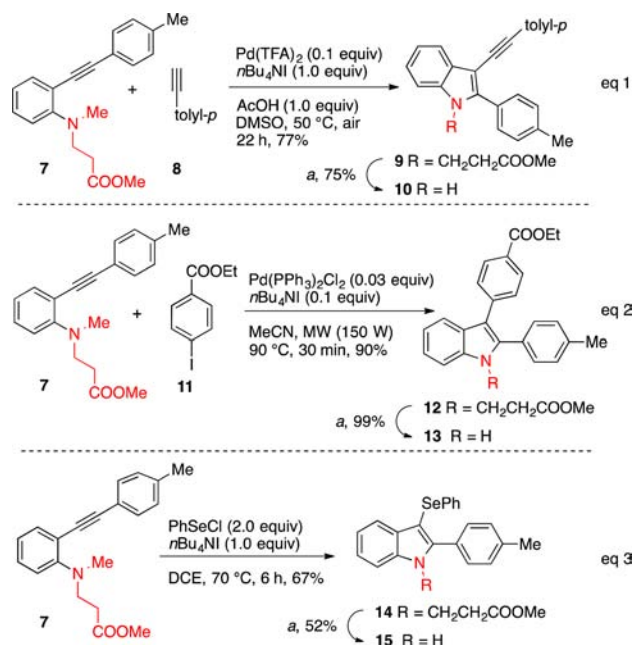
Scheme 4. N -(2-Methoxycarbonyl)ethyl as a Removable Protecting Group in Other Transformations
