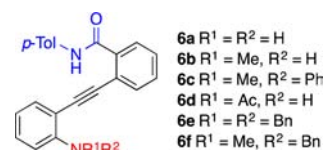
Figure 1. Initial screening of substrates.
