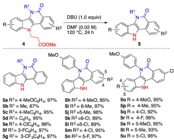
Scheme 3. N -Deprotection of Tetracycles 4 by the Retro-Aza-Michael Addition
