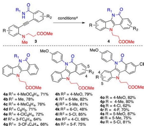
Scheme 2. Synthesis of Tetracycles 4 by Pd-Catalyzed Oxidative Diamination of Alkynes
